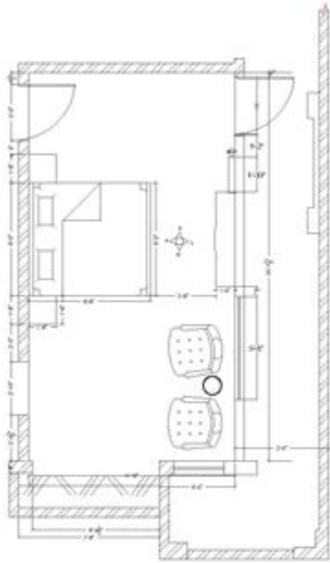
TOP PLAN
