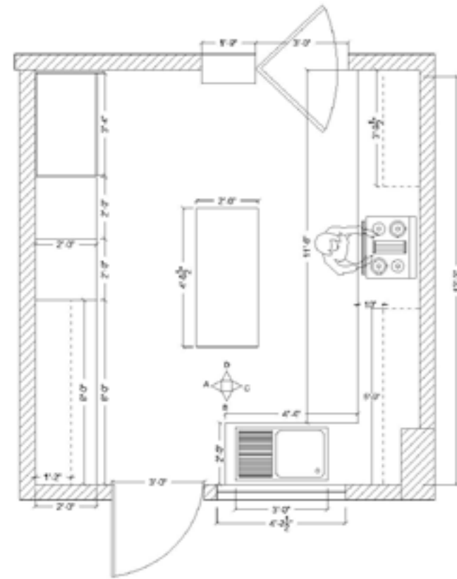
TOP PLAN WASHROOM
